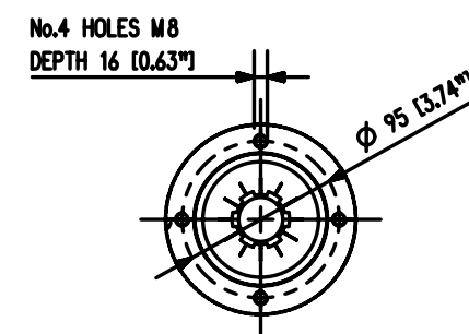
VIEW FROM "W"
